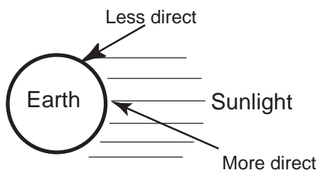
Figure 1. Sunlight striking the Earth.
